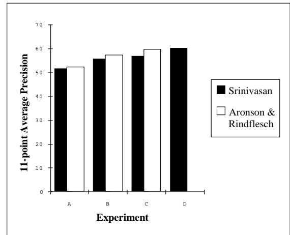
Figure 1. Comparison of Retrieval Results
